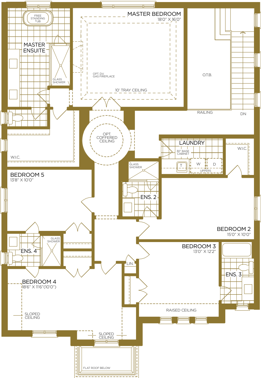
OPT. SECOND FLOOR | ELEV. A 5 BEDROOM
