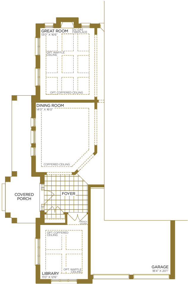
PART. GROUND FLOOR | ELEV. B
