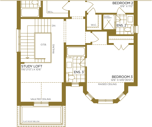
PART. SECOND FLOOR | ELEV. B
