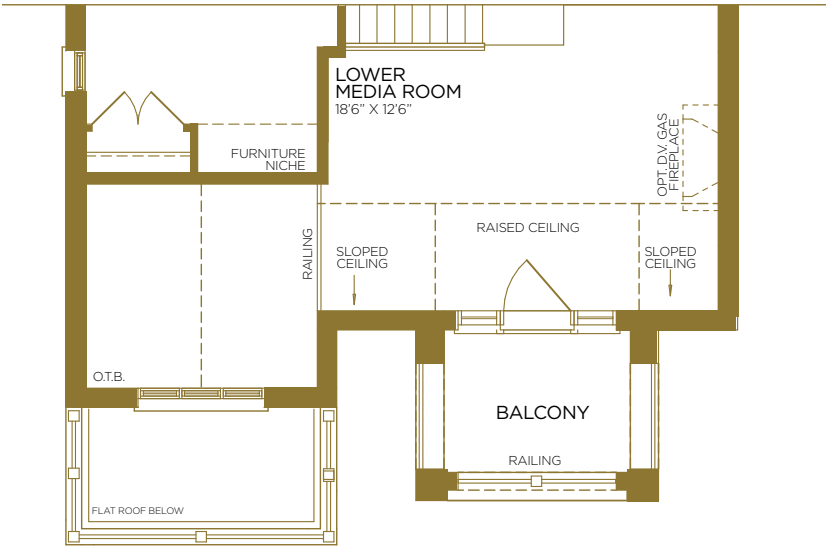
PART. SECOND FLOOR | ELEV. B
