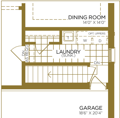
PART. GROUND FLOOR OPT. SERVICE STAIR
