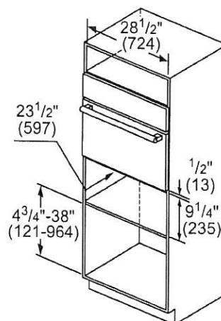
Standard Installation
