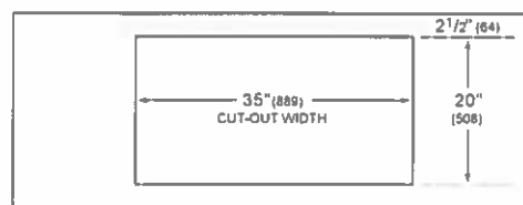
COUNTERTOP CUT-OUT
