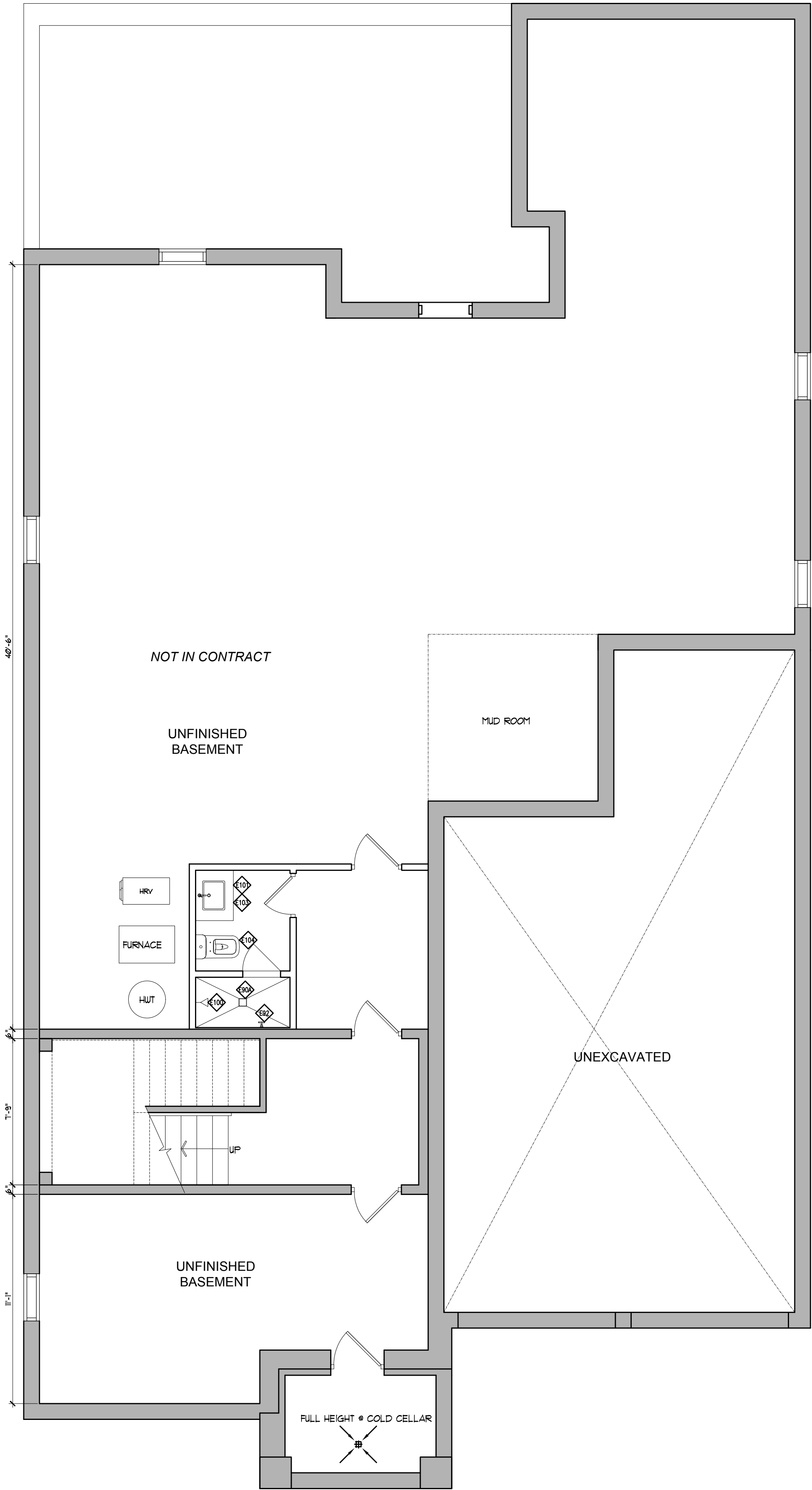
BASEMENT FLOOR PARTITION PLAN SCALE: 1/8" = 1'-0"
