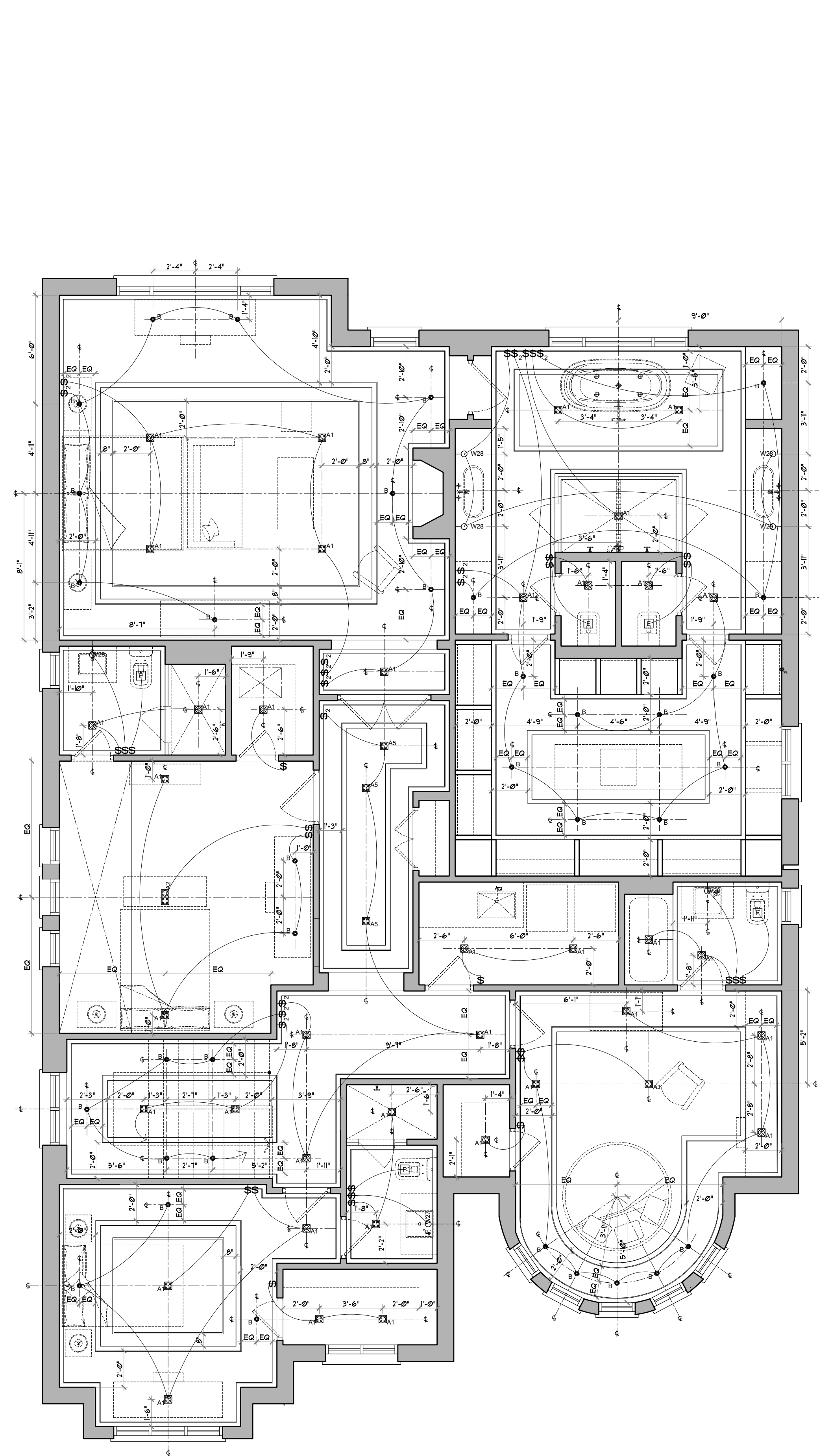
2 SECOND FLOOR REFLECTIVE CEILING PLAN SCALE: 1:50
