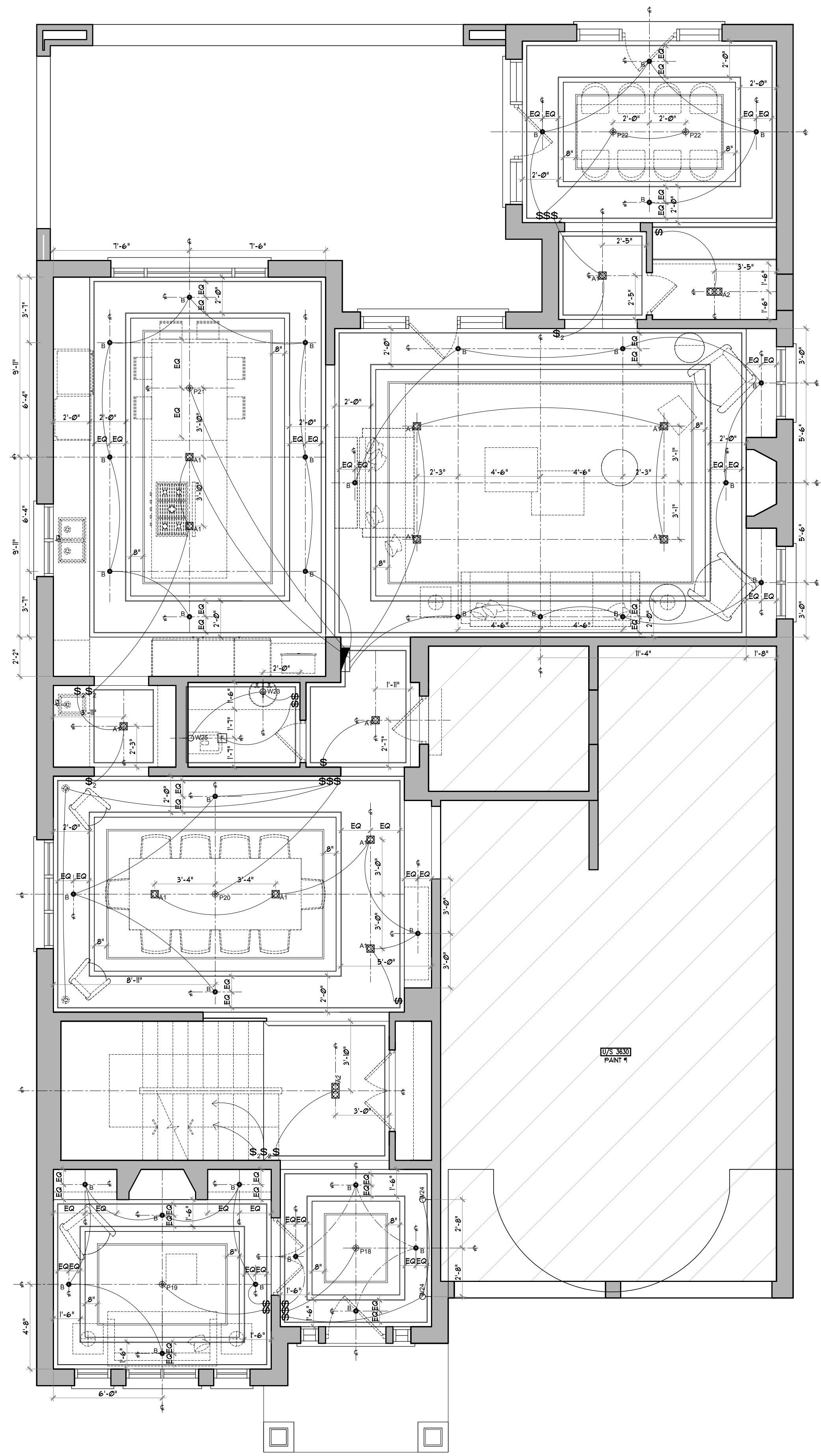
1 FIRST FLOOR REFLECTIVE CEILING PLAN SCALE: 1:50
