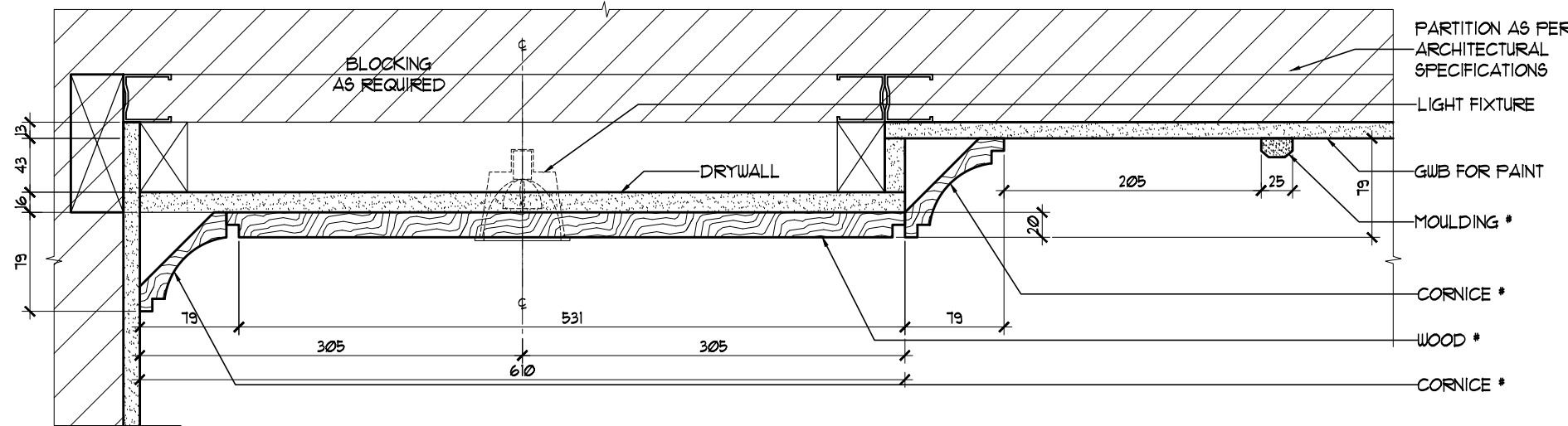
TYP. CORNICE DETAIL VERTICAL SECTION
