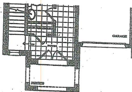
PART. GROUND FLOOR PLAN ELEV. 'C' & 'D'
