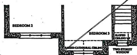
PART. SECOND FLOOR PLAN ELEV. 'B'
