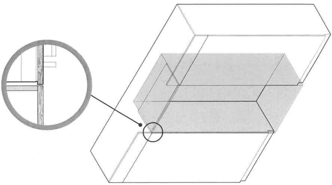
FRAMELESS CABINETY (Aligns the appliance with the cabinetry)
