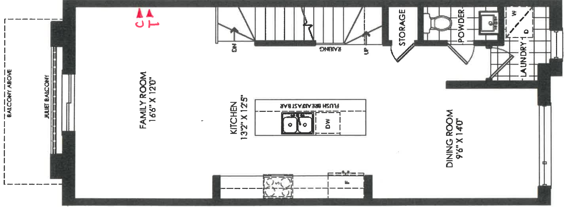
MAIN FLOOR ELEV. 'A'
