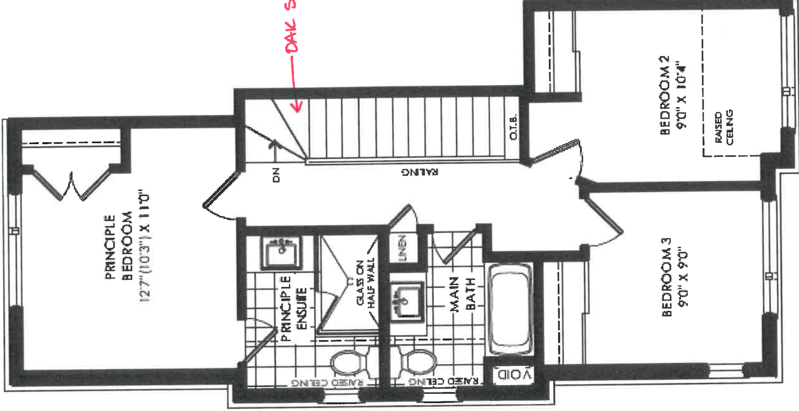
UPPER FLOOR ELEV. 'A'
