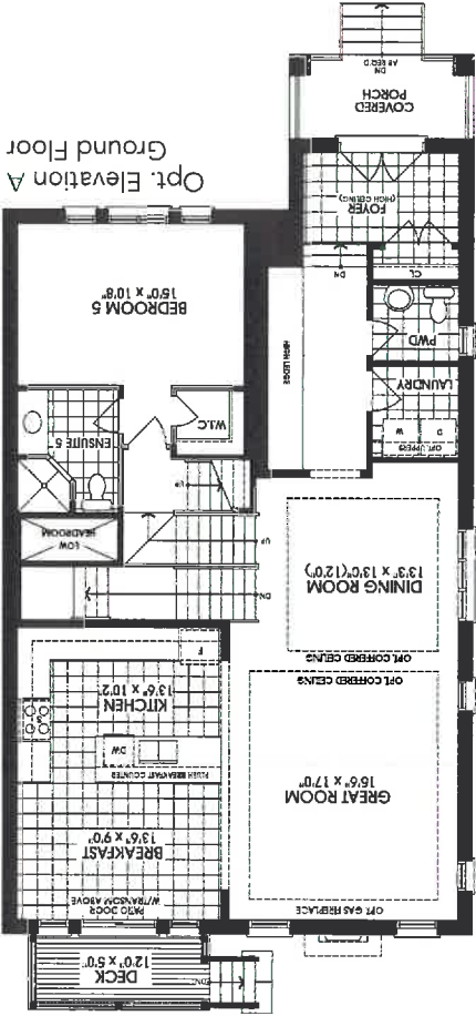
Elevation A Ground Floor
