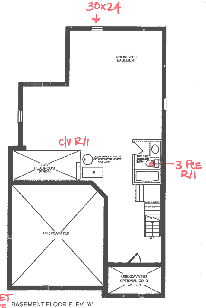
BASEMENT FLOOR ELEV. 'A'
