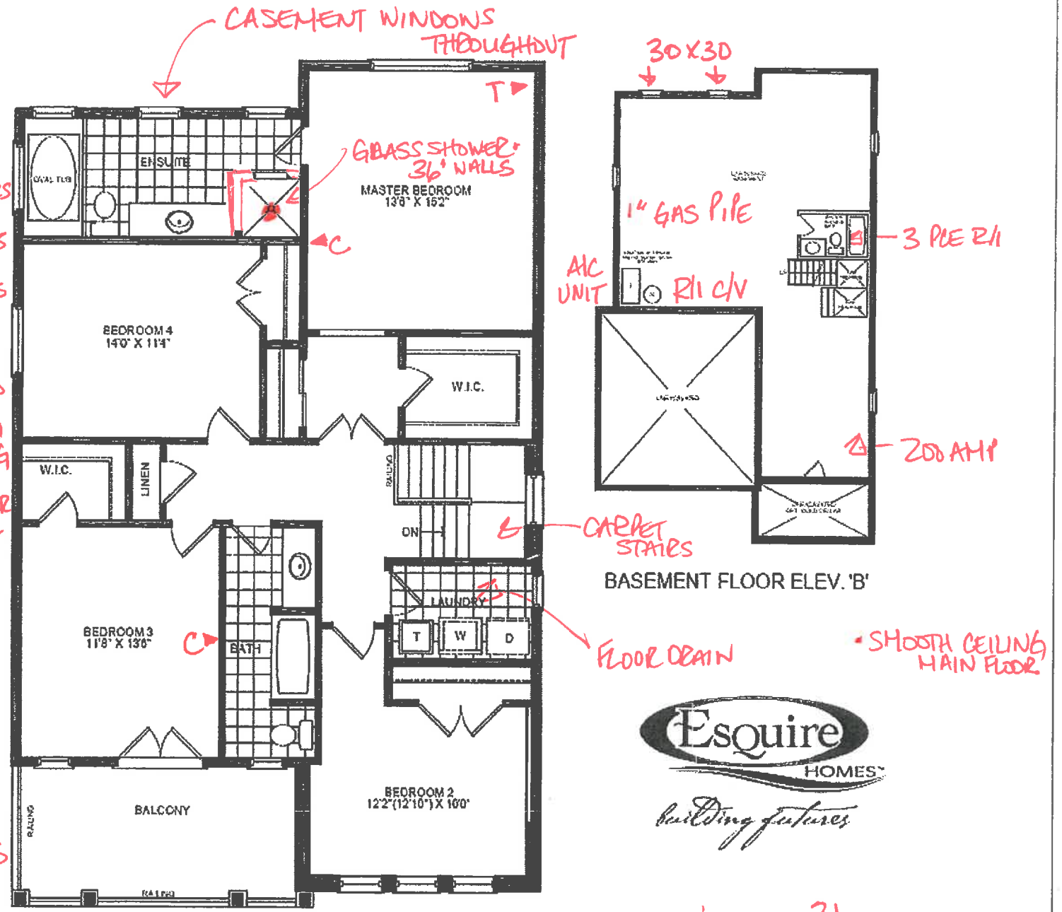
SECOND FLOOR ELEV. 'B'
