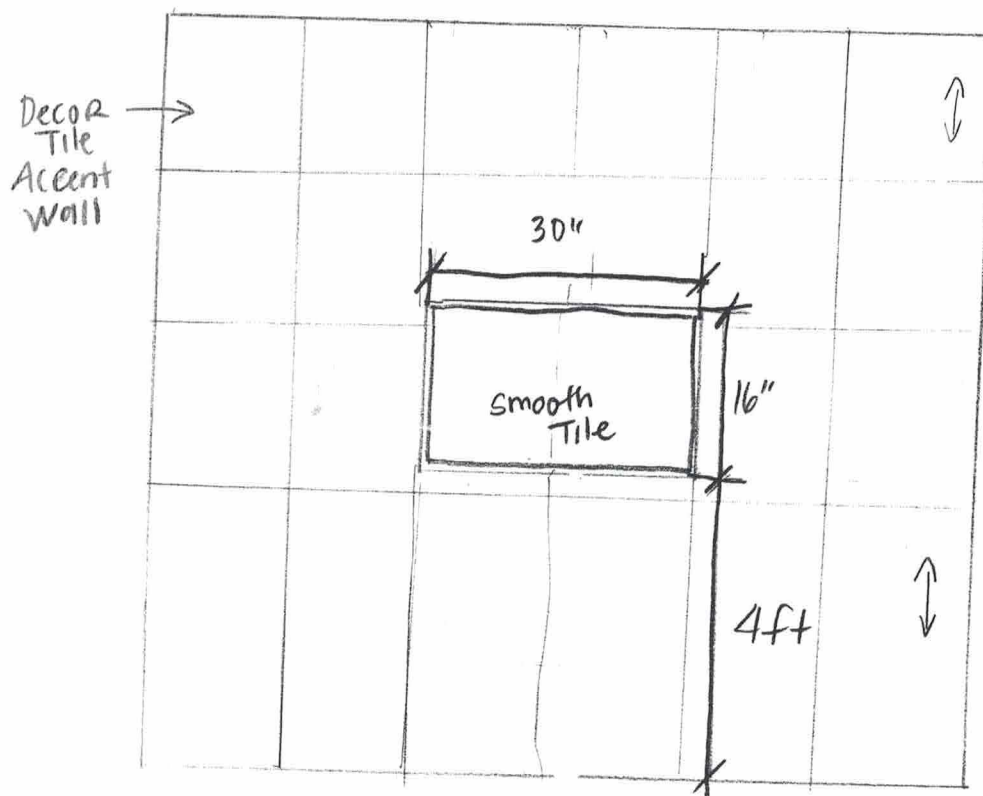
MASTER ENSUITE ELEVATION SHOWER
