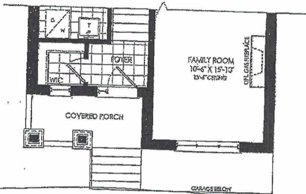
PARTIAL GROUND FLOOR PLAN ELEVATION 'C'
