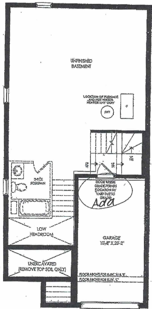
BASEMENT FLOOR PLAN ELEVATION 'A', 'B' & 'C'
