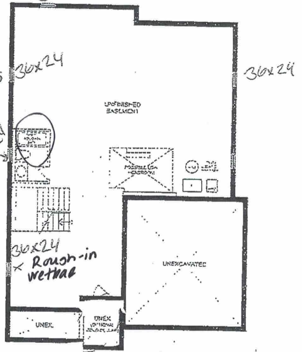
BASEMENT PLAN ELEVATION A
