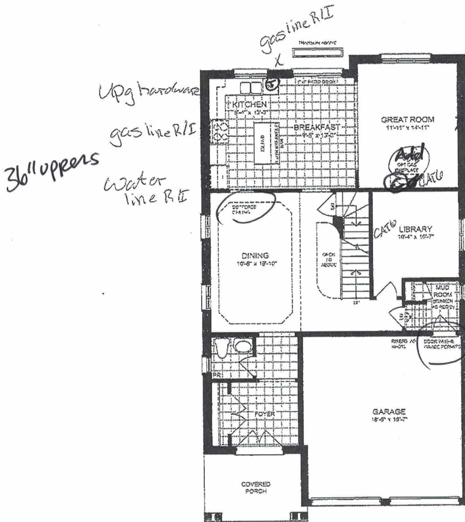
GROUND FLOOR PLAN ELEVATION A
