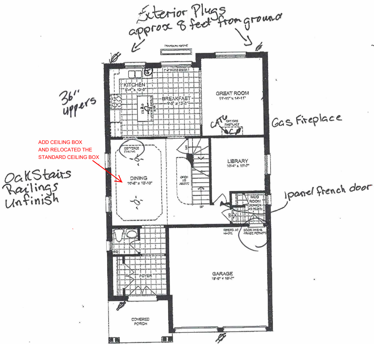
GROUND FLOOR PLAN ELEVATION A
