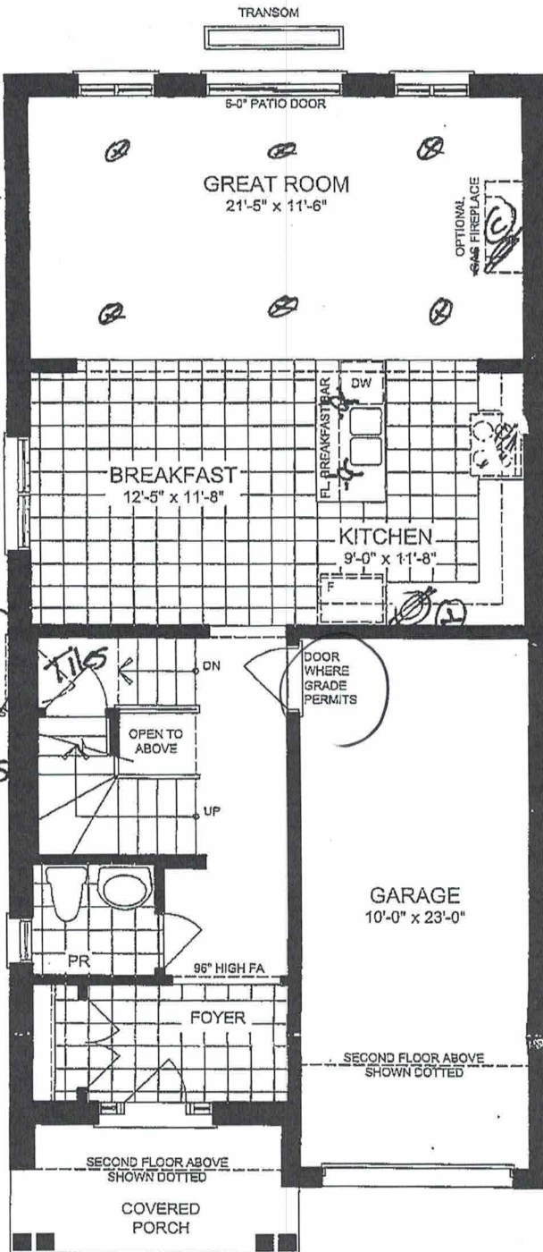
GROUND FLOOR PLAN ELEVATION A & B
