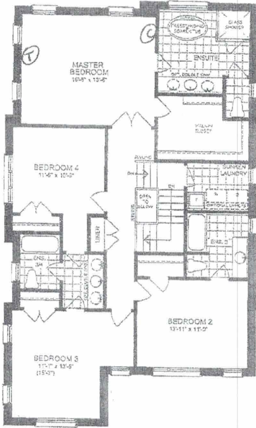
SECOND FLOOR PLAN ELEVATION A
