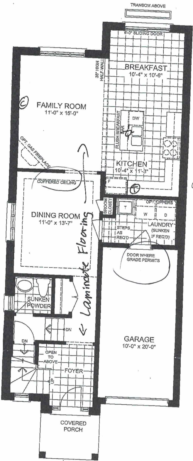
GROUND FLOOR PLAN ELEVATION A & B
