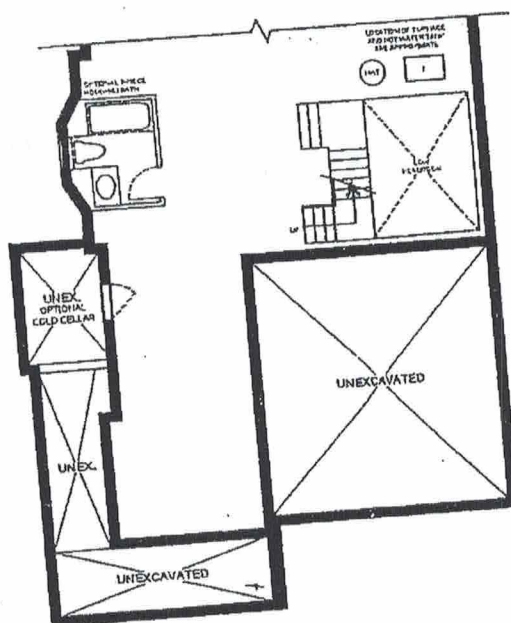
PARTIAL BASEMENT PLAN ELEVATION B
