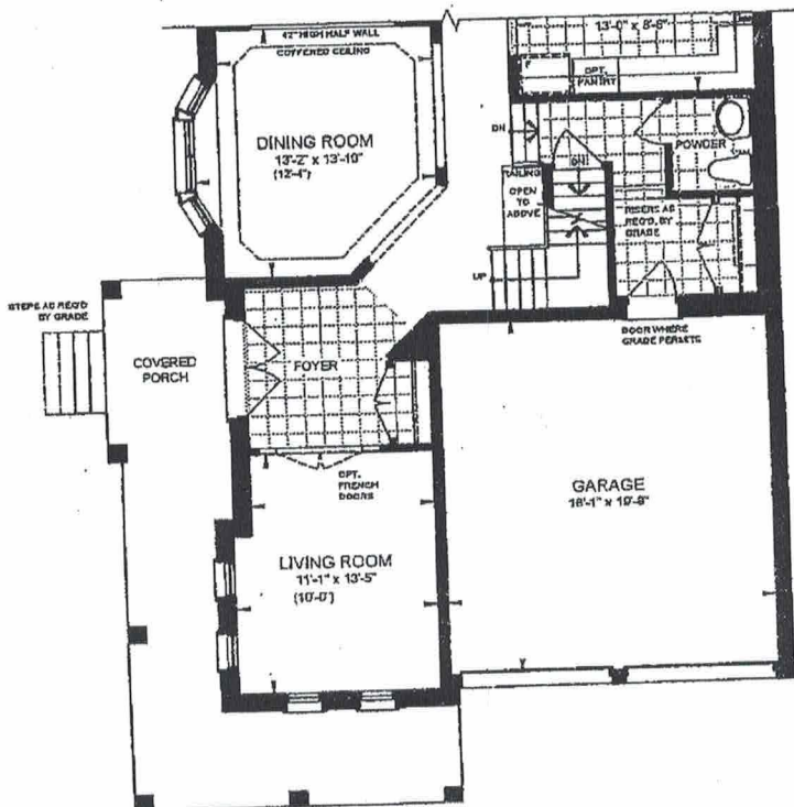
PARTIAL GROUND FLOOR PLAN ELEVATION B
