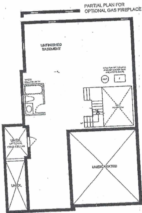
BASEMENT PLAN ELEVATION A
