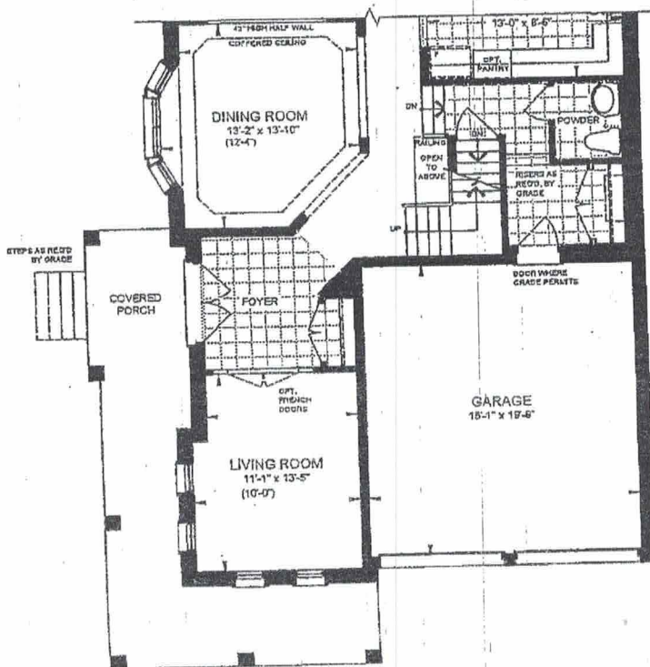
PARTIAL GROUND FLOOR PLAN ELEVATION B
