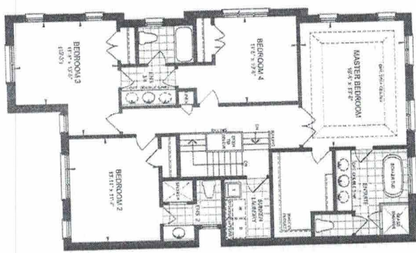
SECOND FLOOR PLAN ELEVATION A
