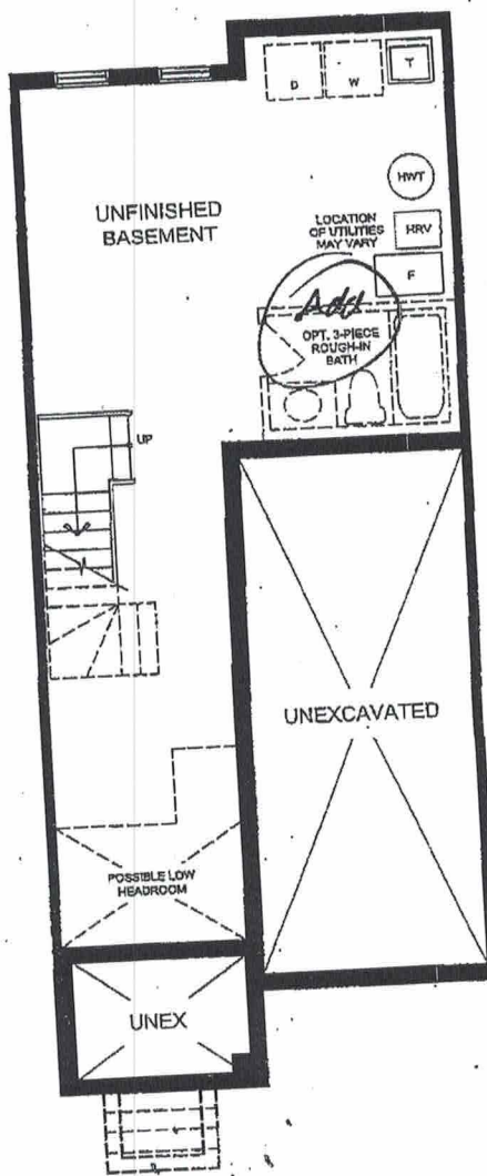
BASEMENT PLAN ELEVATION A
