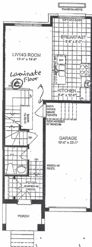
GROUND FLOOR PLAN ELEVATION A
