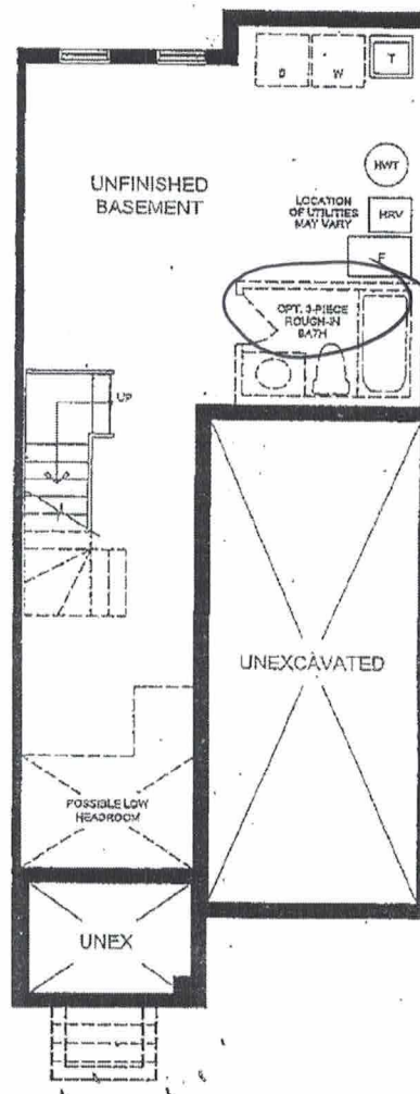
BASEMENT PLAN ELEVATION A
