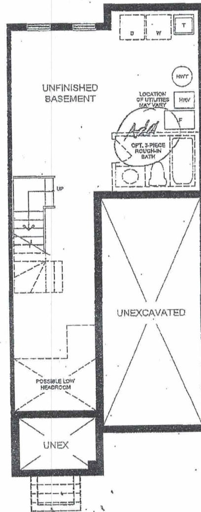
BASEMENT PLAN ELEVATION A
