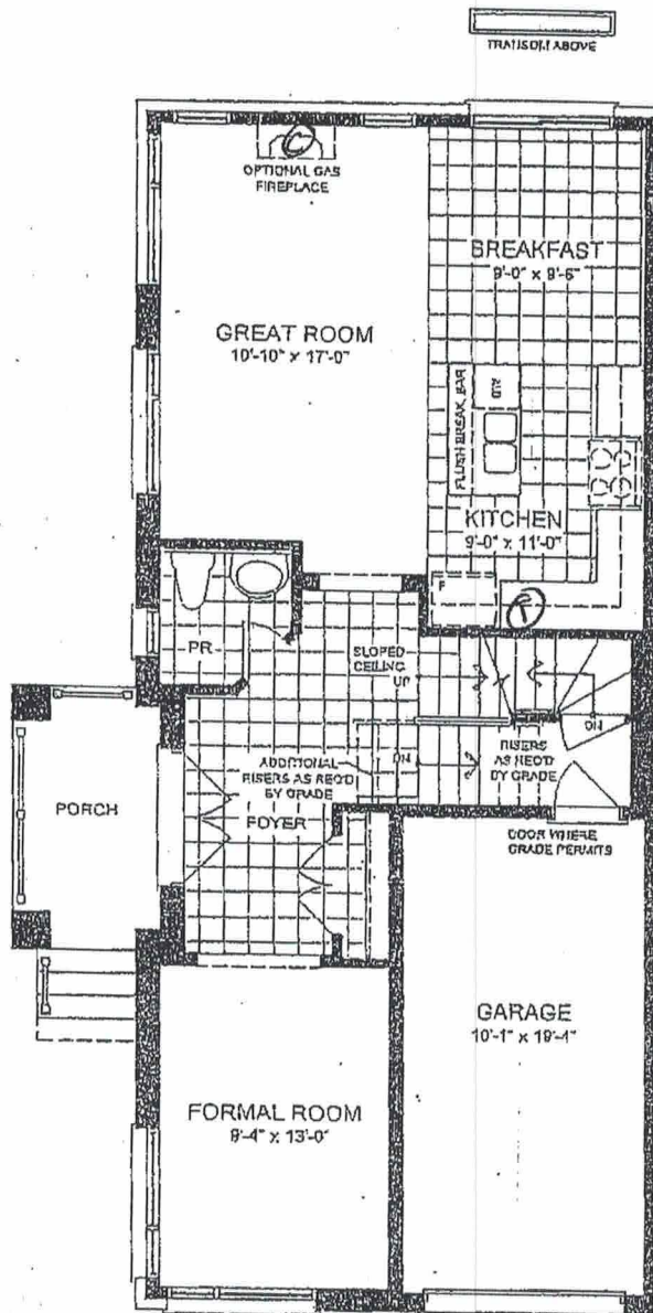
GROUND FLOOR PLAN ELEVATION B
