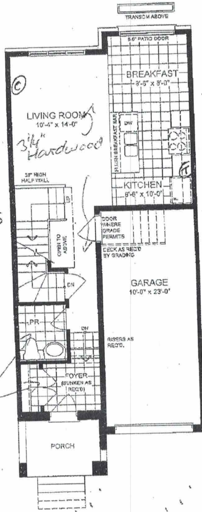
PARTIAL PLAN WITH OPTIONAL GAS FIREPLACE
