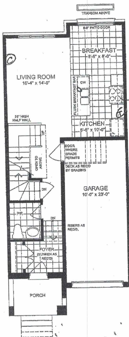
PARTIAL PLAN WITH OPTIONAL GAS FIREPLACE
