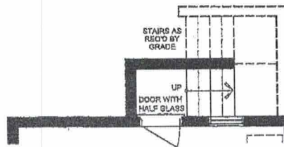
PARTIAL BASEMENT PLAN W/ OPT. WALK-UP
