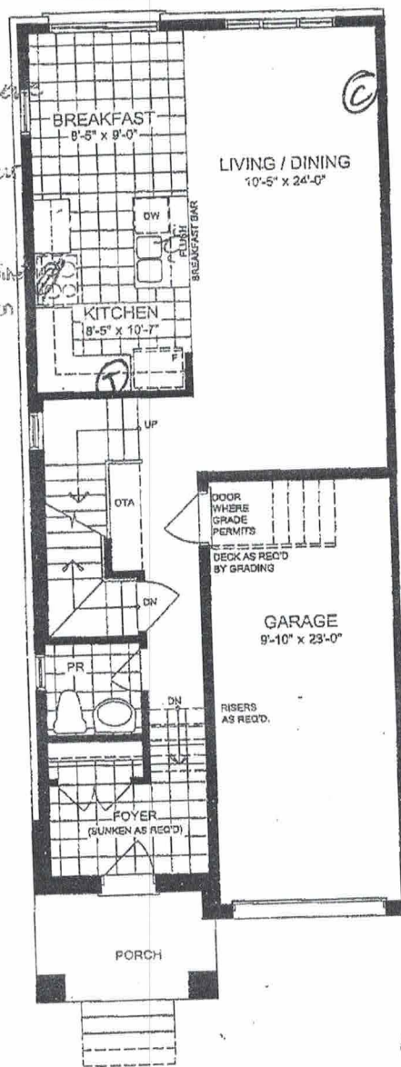
GROUND FLOOR PLAN ELEVATION A
