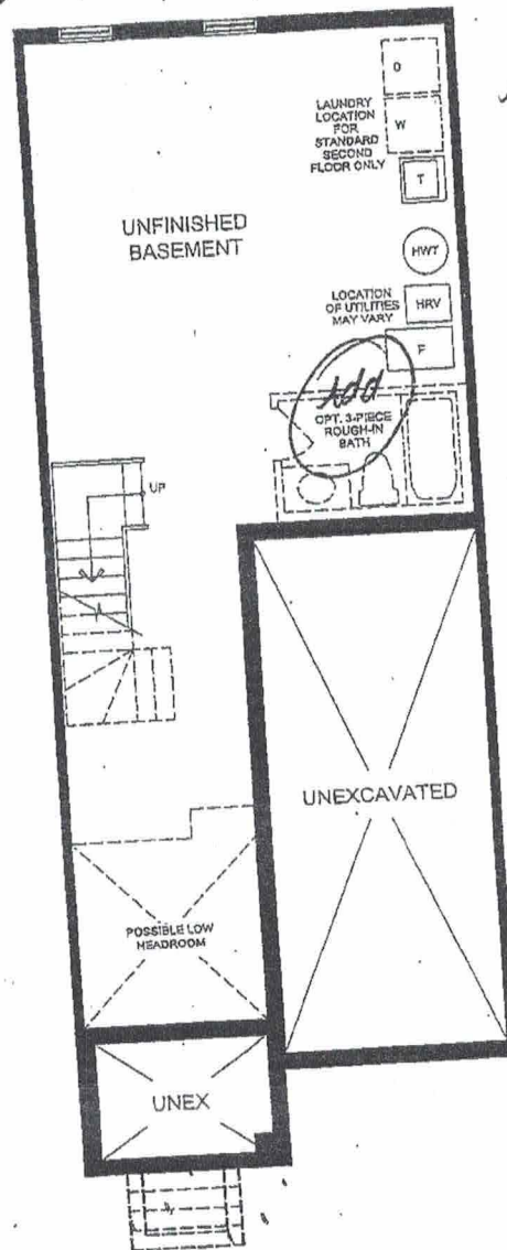
BASEMENT PLAN ELEVATION A
