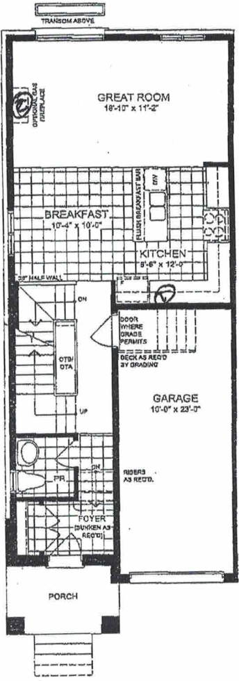
GROUND FLOOR PLAN W/ OPT. FIN. BASEMENT ELEVATION A
