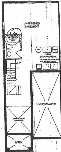
PARTIAL BASEMENT PLAN W/ OPT. WALK-UP
