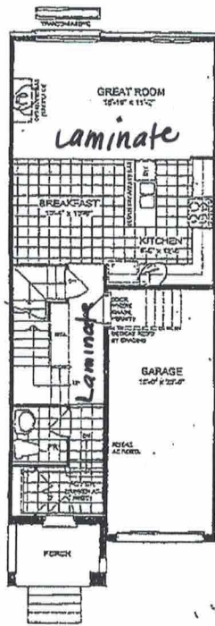
GROUND FLOOR PLAN ELEVATION A
