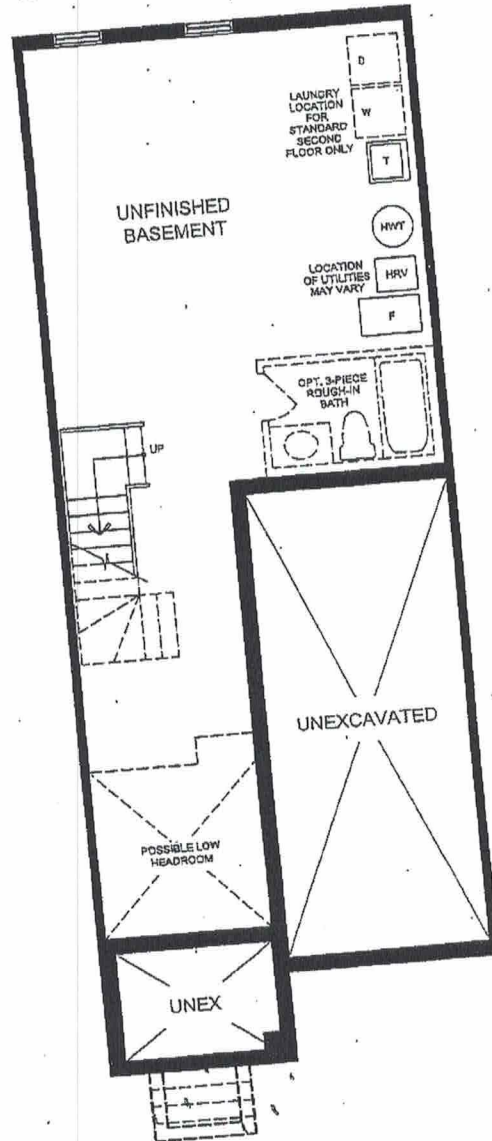
BASEMENT PLAN ELEVATION A
