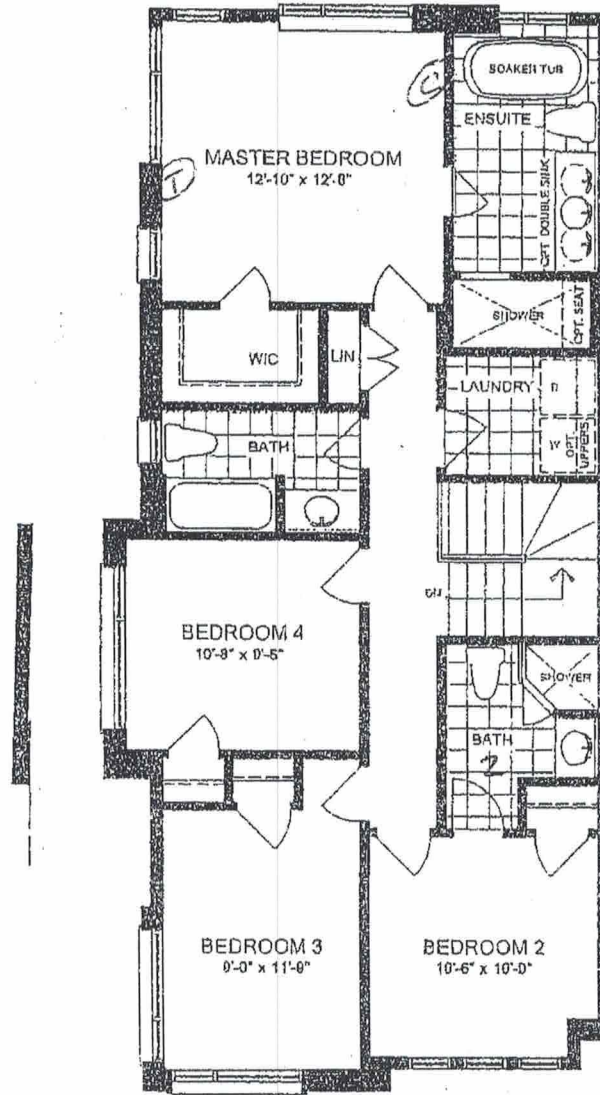
OPTIONAL SECOND FLOOR PLAN ELEVATION A
