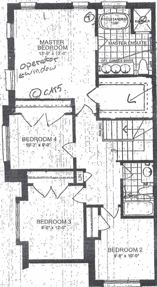
SECOND FLOOR PLAN ELEVATION B
