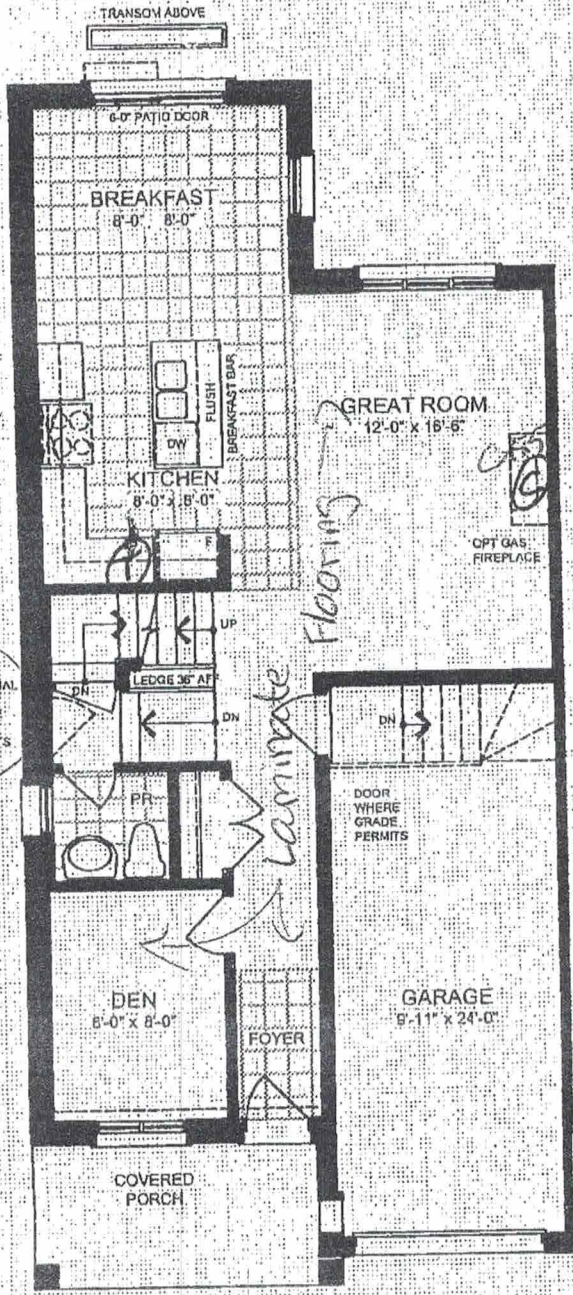
GROUND FLOOR PLAN ELEVATION A1, A2, & B
