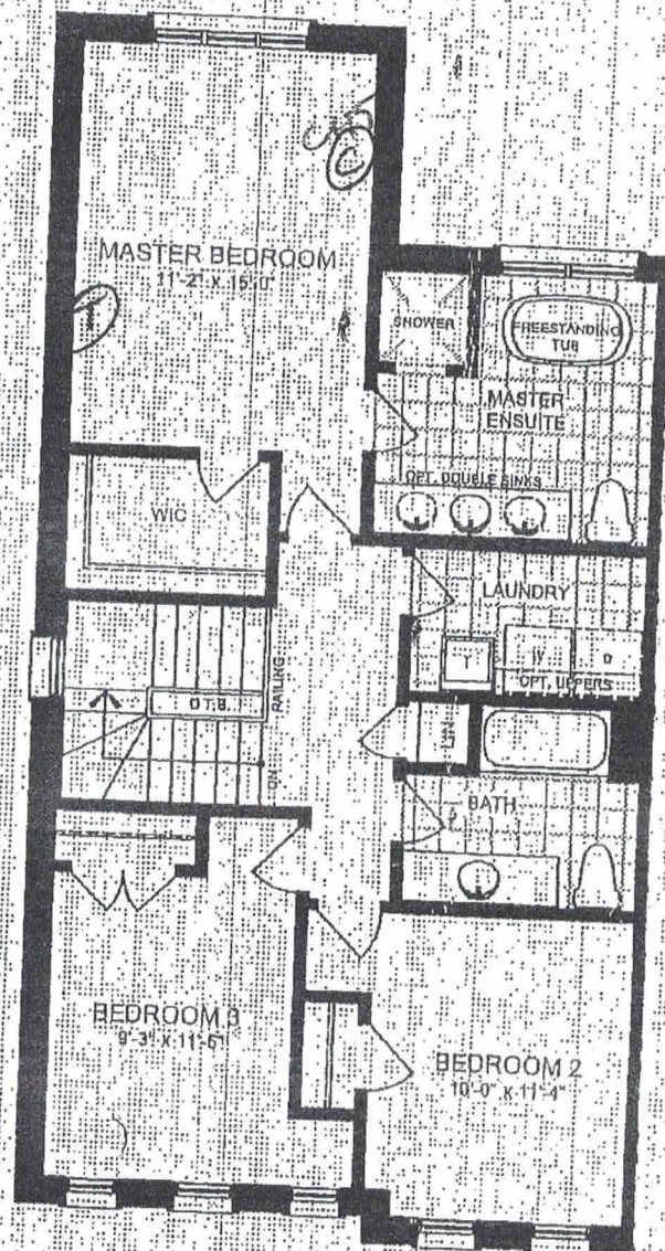
SECOND FLOOR PLAN ELEVATION A1
