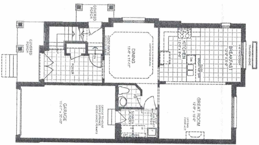
GROUND FLOOR PLAN ELEVATION B
