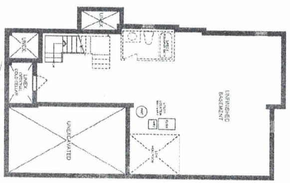
BASEMENT PLAN ELEVATION B
