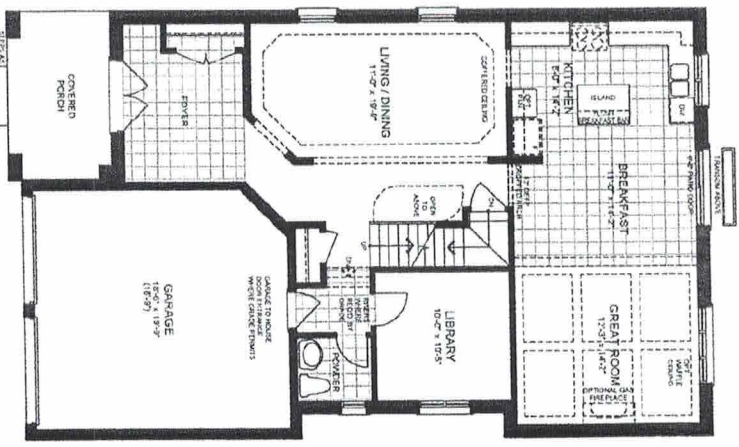
GROUND FLOOR PLAN ELEVATION A
