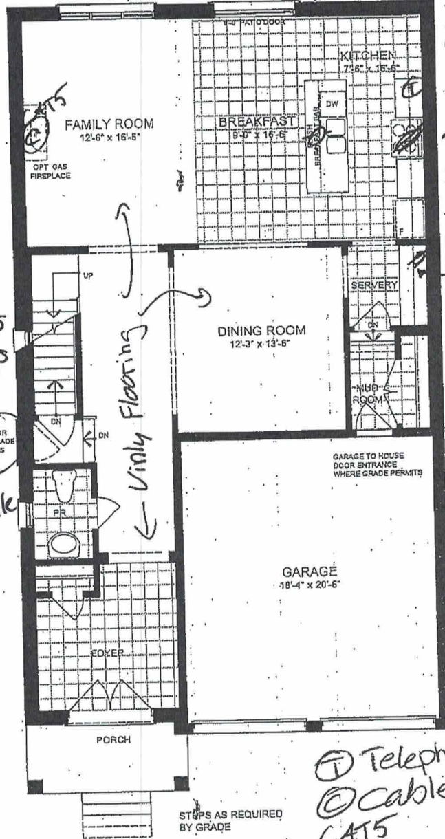
GROUND FLOOR PLAN ELEVATION A
