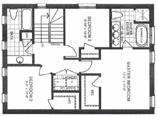
SECOND FLOOR PLAN ELEVATION A
