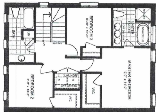
SECOND FLOOR PLAN ELEVATION A
