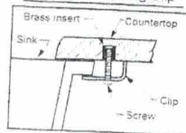
Detail of Mounting Clip
