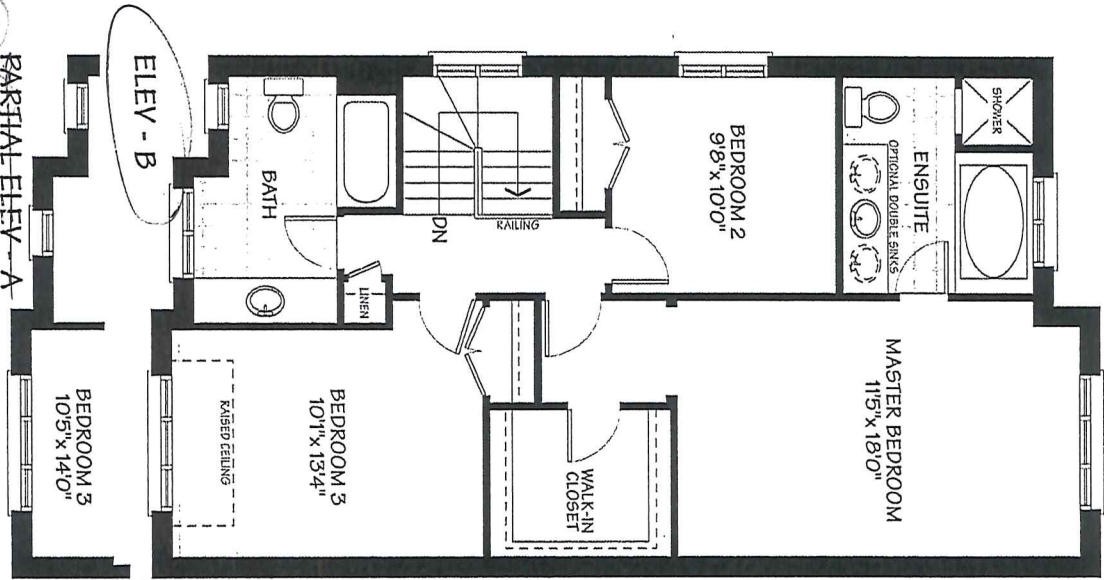
SECOND FLOOR
