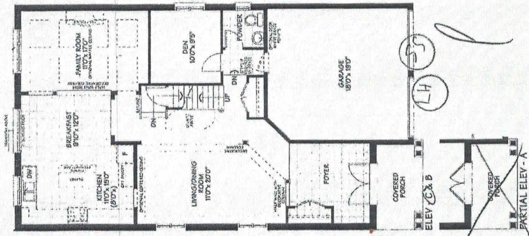
MAIN FLOOR
